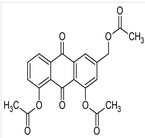
Chemical Structure - Triacetyl aloë-emodin (Impurity A), Aloe-emodin derivative (ab145181)
